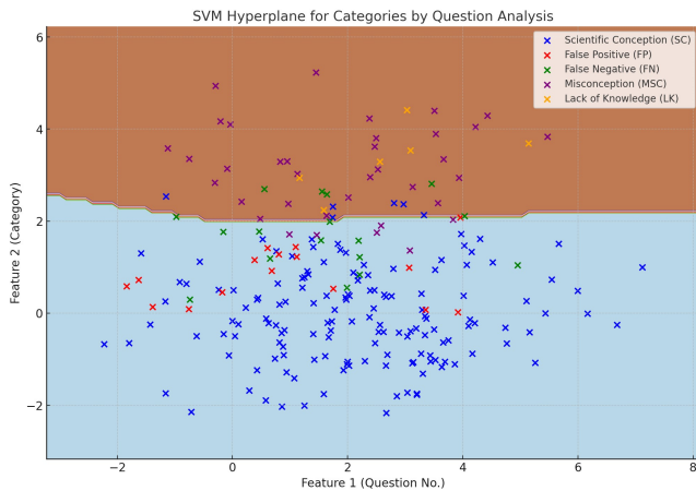
Fig. 12. SVM hyperplane visualization for categorizing student responses by question analysis.
