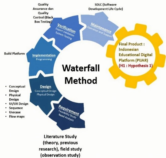
Fig. 2. Stages of waterfall method.
