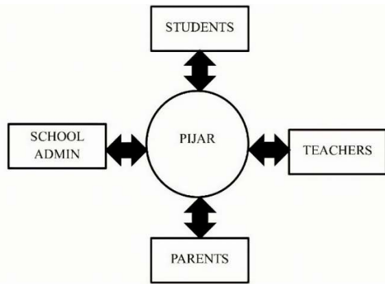
Fig. 4. Context diagram.
