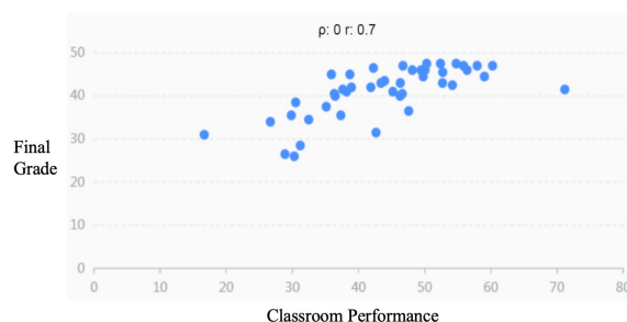
Fig. 4. The student data analytics of TMT.
