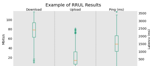
Fig. 4. Example of RRUL boxplot.
