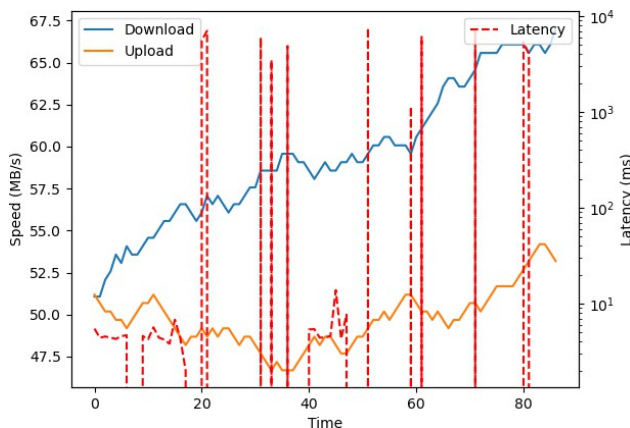
Fig. 8. DoS attack during portions of training without causing failure.
