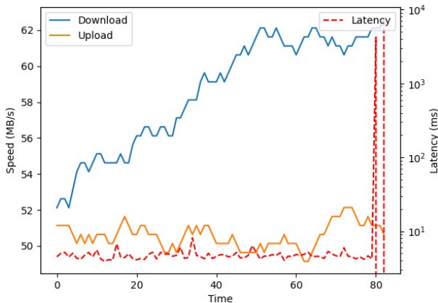
Fig. 7. DoS attack during training: Note the spike in latency towards the end, followed by the training crash.
