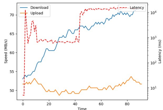
Fig. 6. Example of a DoS attack sustained throughout training.
