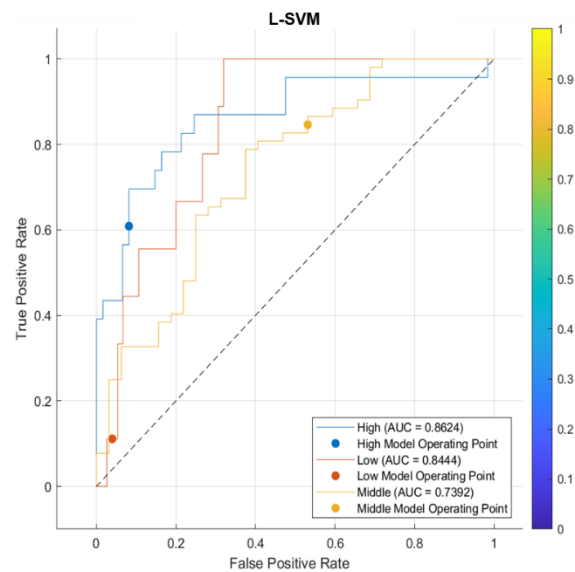
Fig. 4. AUC-ROC Curve of L-SVM.
