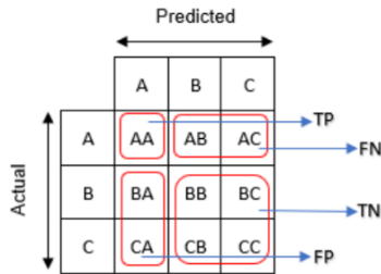
Fig. 2. Confusion matrix 3×3 [31].
