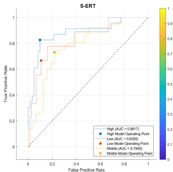
Fig. 9. AUC-ROC Curve of S-ERT.
