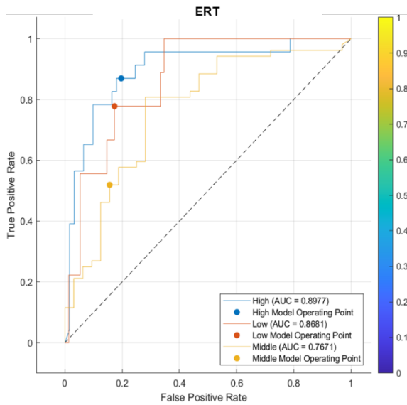
Fig. 8. AUC-ROC Curve of ERT.
