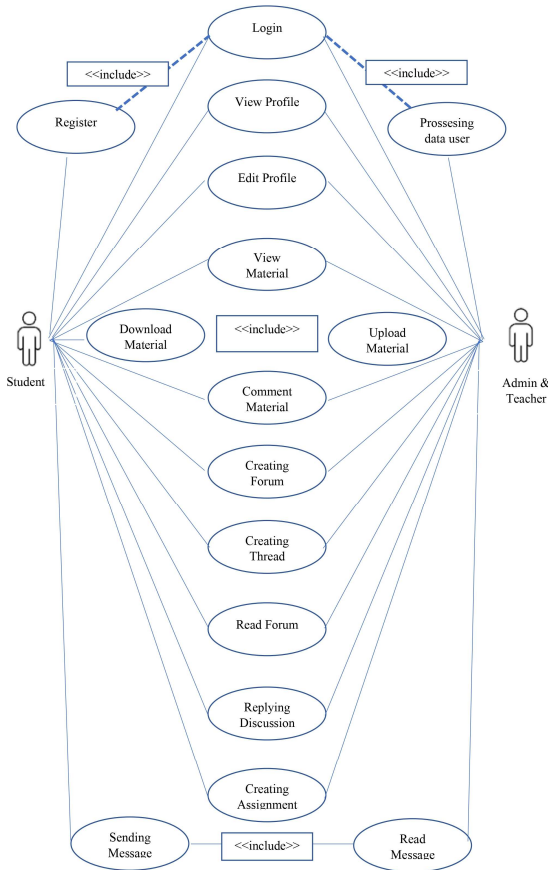
Fig. 2. Use case design.
