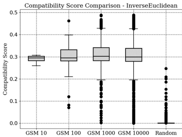
Fig. 9. The boxplot graph shows the pairing distributions using inverse Euclidean compatibility scores on numerical and categorical datasets.
