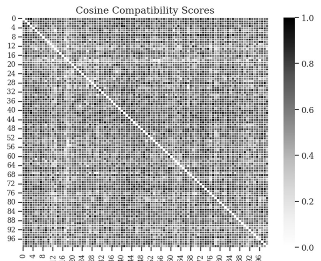
Fig. 5. Heatmap cosine compatibility scores.
