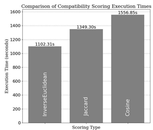
Fig. 1. Graph of execution time for compatibility scoring (numerical data).
