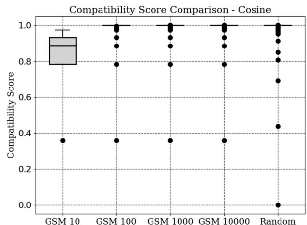
Fig. 11. Boxplot pairing distributions graph using Cosine compatibility scores on numerical and categorical datasets.
