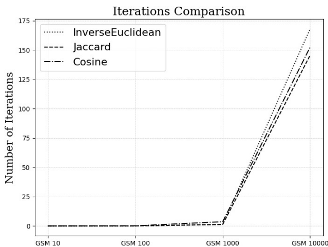
Fig. 13. Comparison of iterations in pair formation for inverse Euclidean, Jaccard and Cosine compatibility metrics.
