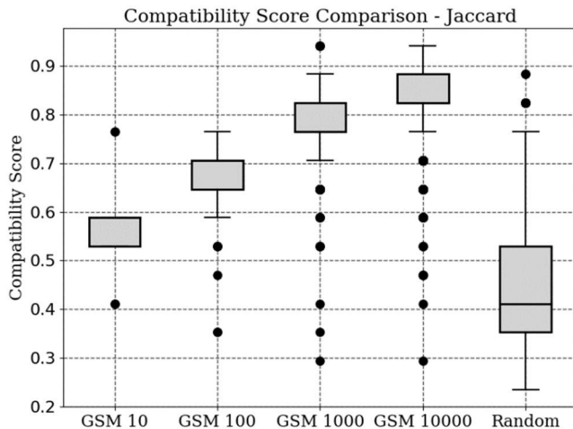
Fig. 10. The boxplot graph illustrates the pairing distributions using Jaccard compatibility scores on numerical and categorical datasets.
