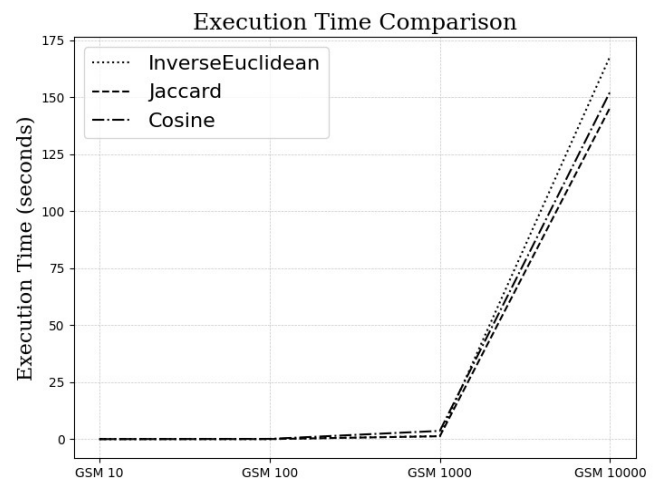
Fig. 12. Comparison of execution time in pair formation for inverse Euclidean, Jaccard and Cosine compatibility metrics.
