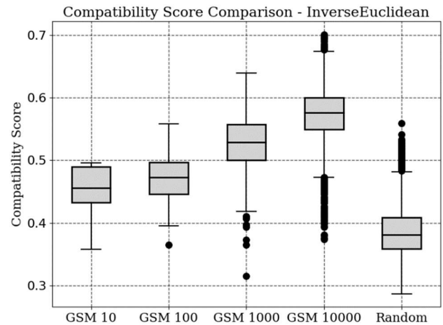
Fig. 6. The boxplot graph illustrates the pairing distributions using inverse Euclidean compatibility scores on the numerical dataset.
