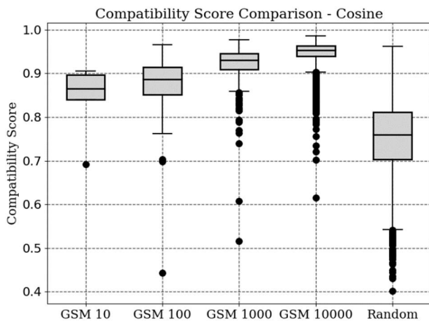
Fig. 8. Boxplot pairing distributions graph using Cosine compatibility scores on the numerical dataset.
