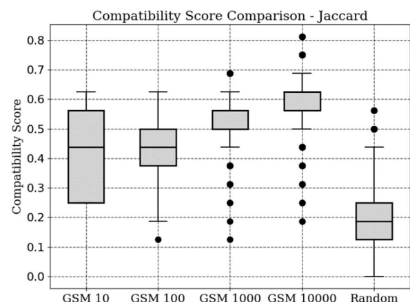
Fig. 7. The boxplot graph displays the pairing distributions using Jaccard compatibility scores on the numerical dataset.
