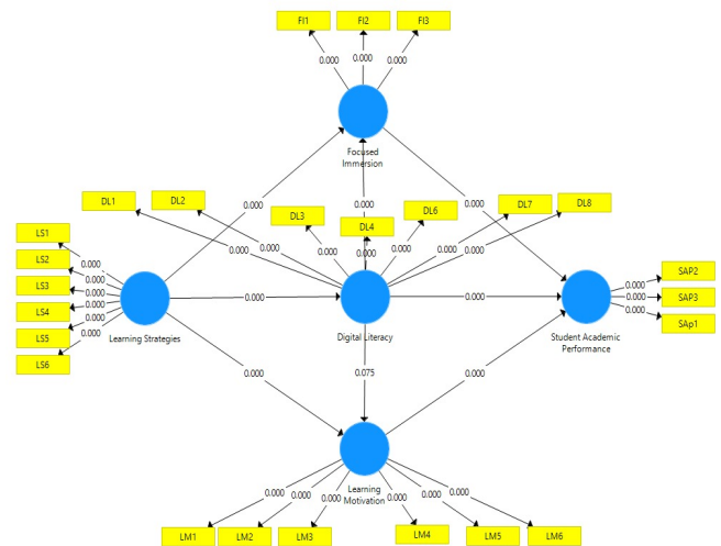
Fig. 3. Model Calculation Results with P-Value (SmartPLS 3).
