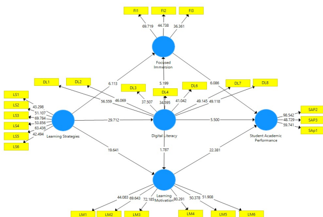
Fig. 2. Model Calculation Results with T values (Smart PLS 3).
