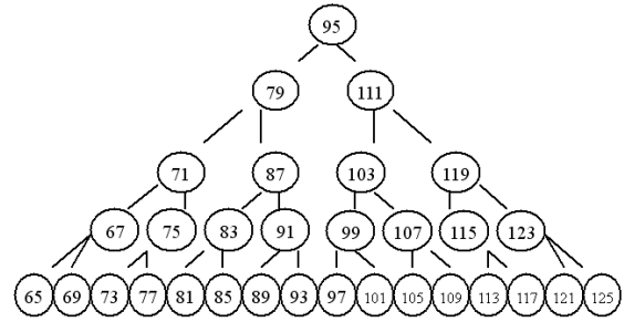
Fig. 9. Interval tree constructed from odd interval [65, 125].
