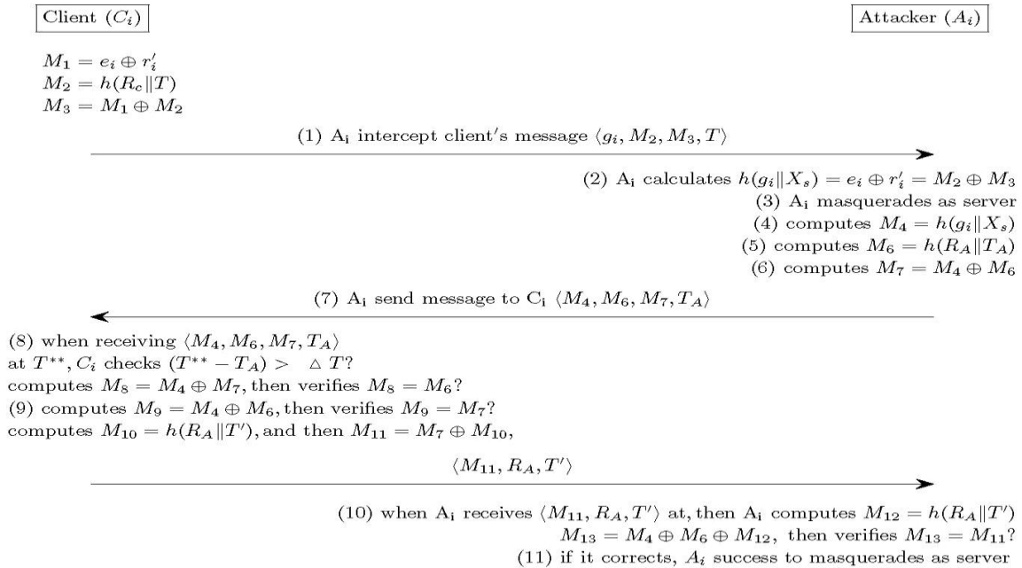
Fig. 4. Server masquerading attack.
